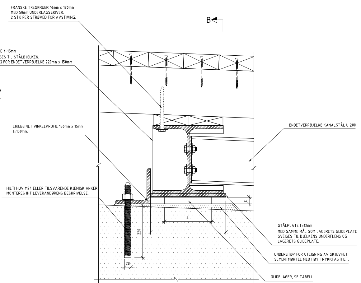
DETALJ OPPLEGG 1:10
